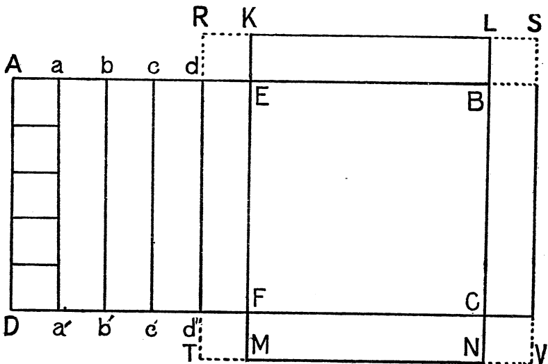
FIG. 6.—EVALUATION OF \sqrt{5000} (RASHI'S METHOD).
